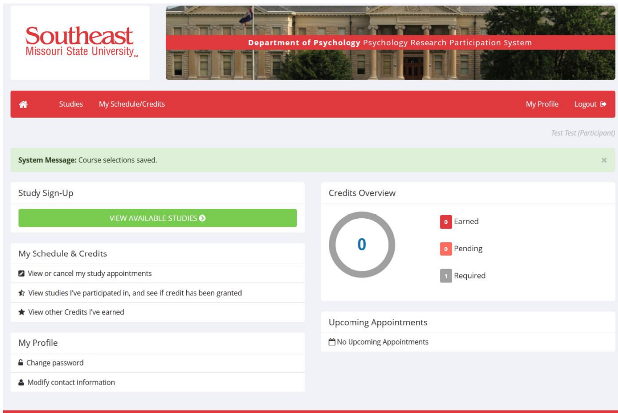
Figure 2 - Main Menu
